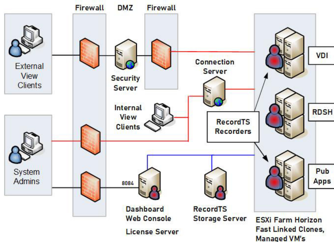
RecordTS v5 for VMWare Horizon View Network Configuration
