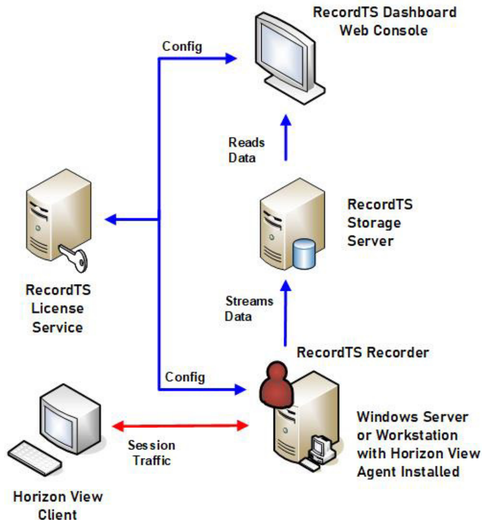
RecordTS v5 for VMware Horizon 7 Functional Diagram
